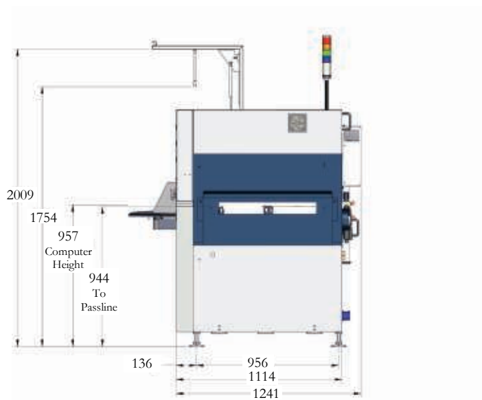
Side View (mm)
