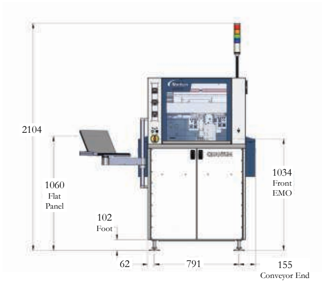
Front View (mm)
